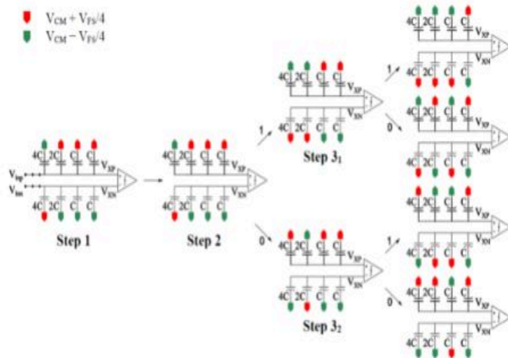
Figure 7. Traditional switching technique of a 3-bit SAR ADC
