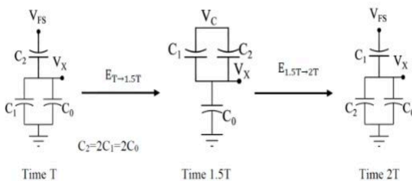
Figure 6. Charge Redistribution Technique for Two Capacitor Switching in opposite polarity
