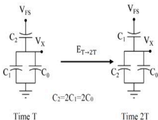
Figure 5. Single capacitor switching.
